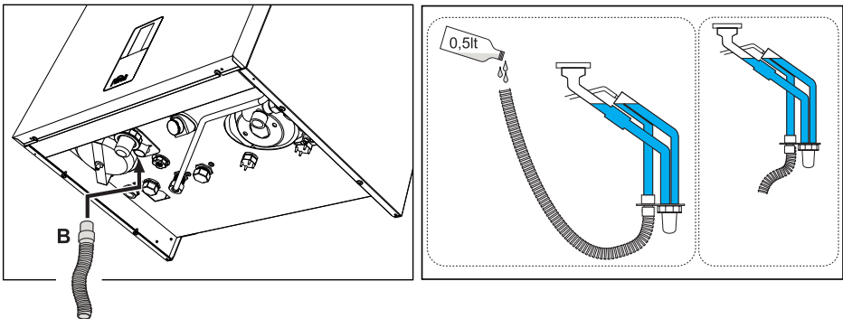
fig. 37- Condensate drain connection
