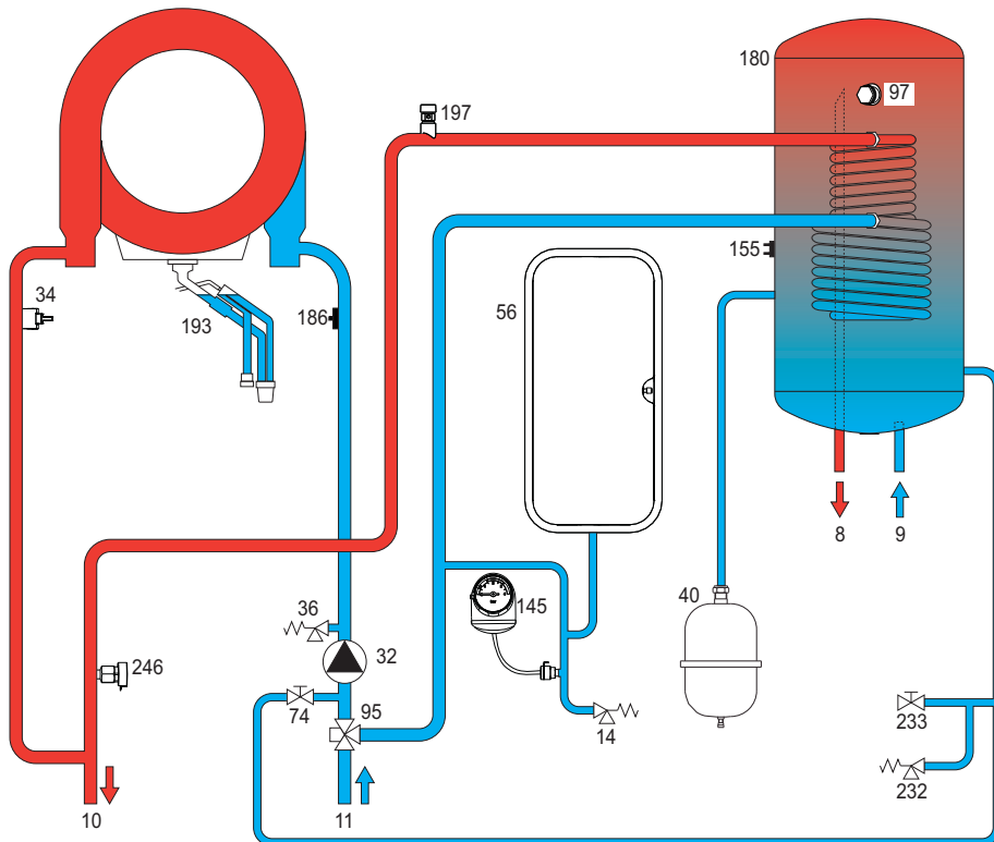
fig. 48- Hydraulic circuit
