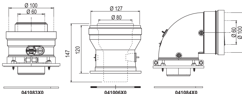
fig. 31- Starting accessories for coaxial ducts
