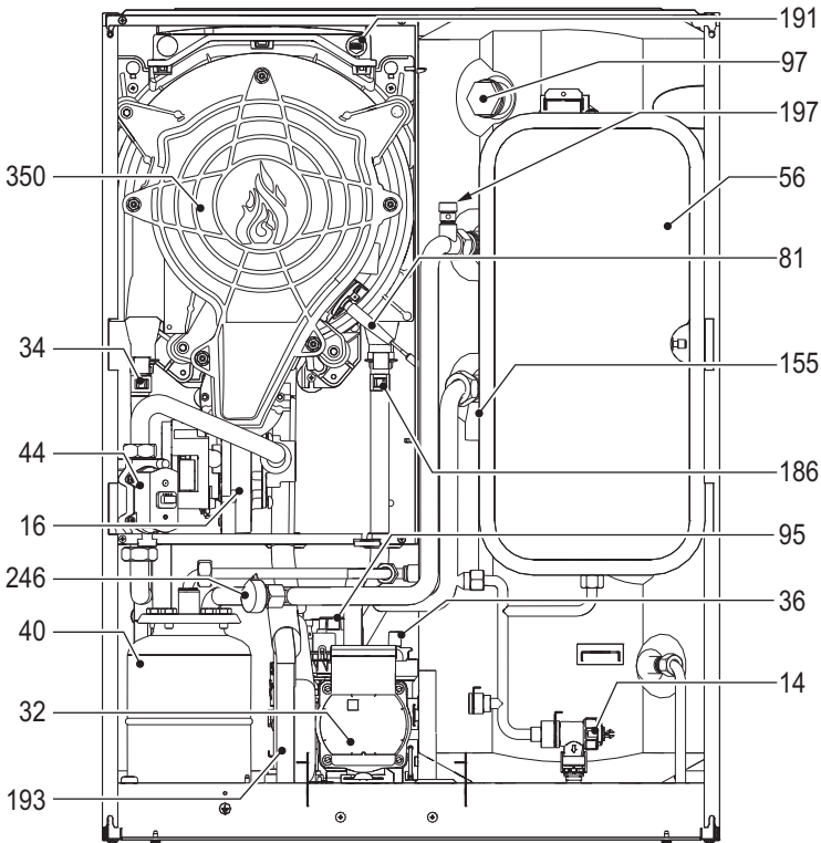
fig. 47- General view
