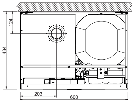
fig. 45- Top view
