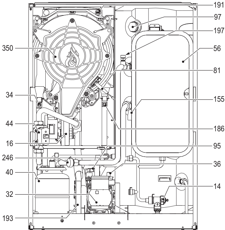
fig. 47- Vista general
