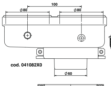
fig. 33- Starting accessory for separate ducts
