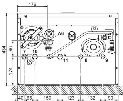
fig. 46- Bottom view
