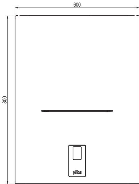
fig. 43- Front view
